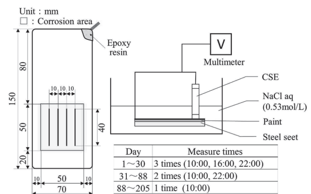
Fig. 1 Specimen and electrochemical test on painted steel sheet
