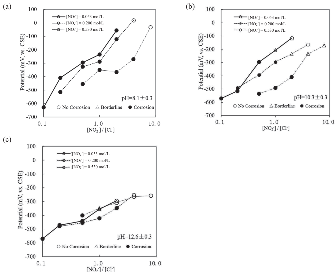
Fig. 4 Effect of [\text{NO}_2^-]/[\text{Cl}^-] molar ratio on the corrosion potential of steel
